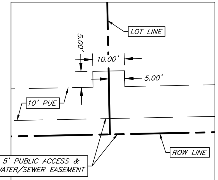
Typical 5'x10' Easement Extension N.T.S.
